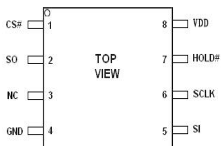
SOP8-B
