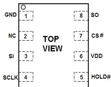
DFN8 2X3
