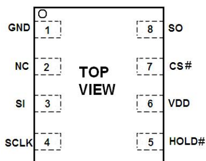
DFN8 2X3
