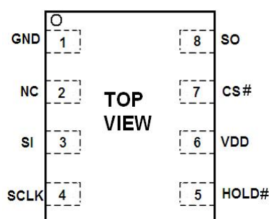
DFN8 5X6
