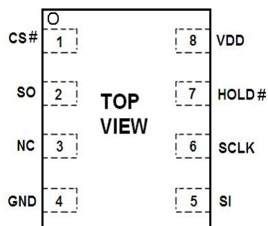
WSN 5X6
